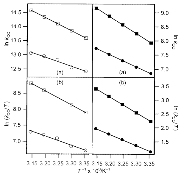
Fig. 5 (a) Arrhenius and (b) Eyring plots obtained for the reaction of \text{Mn}(\eta^5\text{-C}_5\text{H}_5)(\text{CO})_2(n\text{-C}_7\text{H}_{16}) ( \square ), \text{Mn}(\eta^5\text{-C}_5\text{H}_5)(\text{CO})_2(\text{C}_5\text{H}_{10}) ( \circ ), \text{Re}(\eta^5\text{-C}_5\text{H}_5)(\text{CO})_2(\text{C}_5\text{H}_{10}) ( \bullet ) and \text{Re}(\eta^5\text{-C}_5\text{H}_5)(\text{CO})_2(n\text{-C}_7\text{H}_{16}) ( \blacksquare ) with CO.
